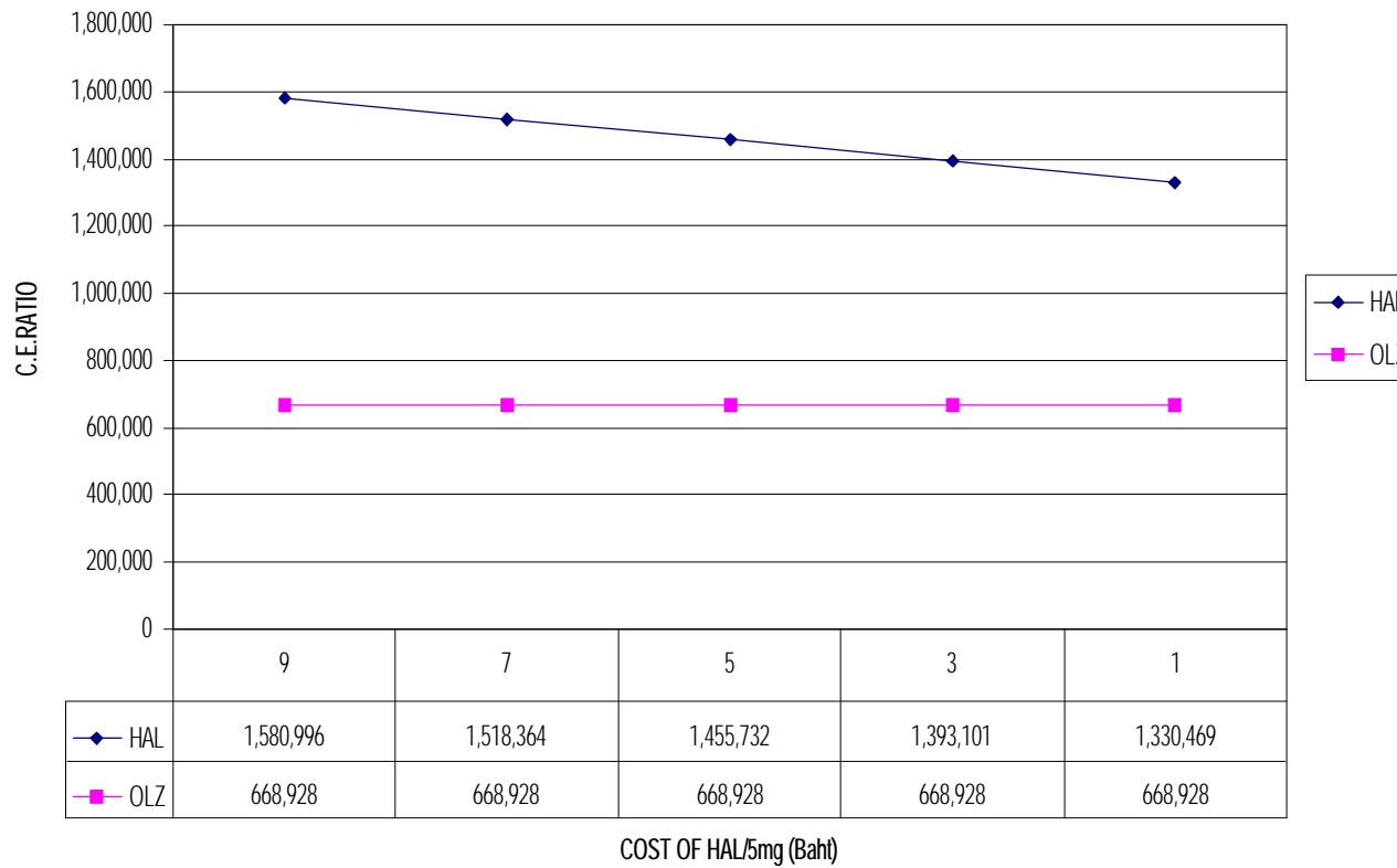
Figure 4. Sensitivity analysis on cost of haloperidol
