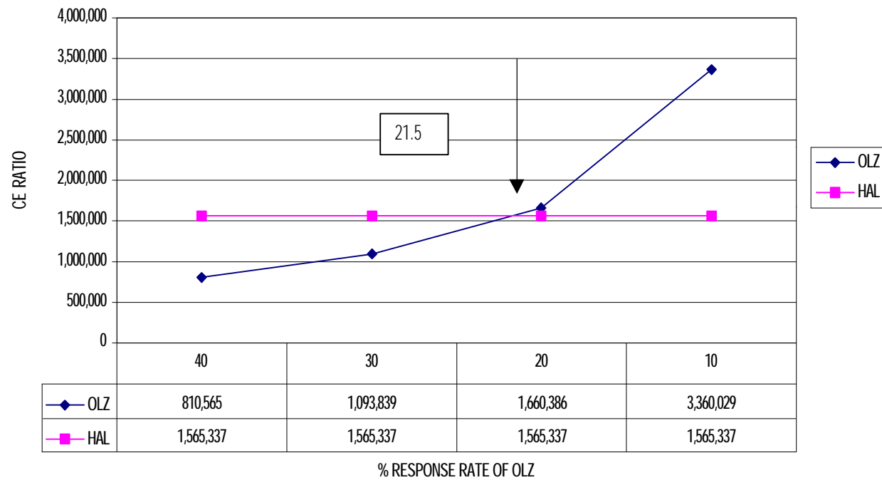
Figure 2. Sensitivity analysis on response rate of olanzapine
