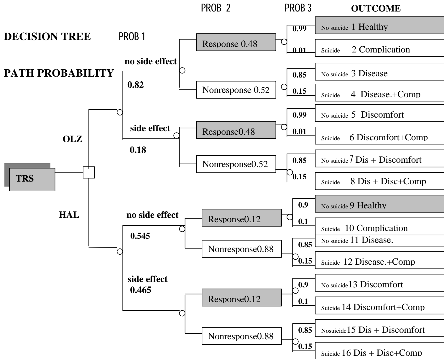
FIGURE 1. Decision tree of the analysis
